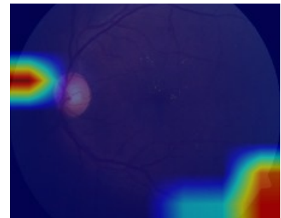
Overlay
