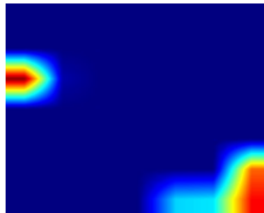
Grad-CAM
